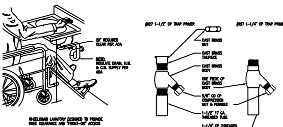
TYPICAL HANDICAPPED WALL MOUNTED LAVATORY DETAIL N.T.S.
