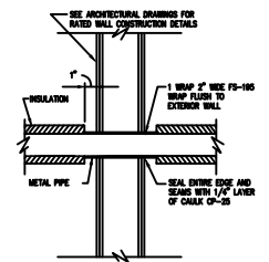
TYPICAL WALL TYPE FIRESTOP DETAIL N.T.S.
