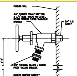
TYPICAL INTERIOR HOSE BIBB DETAIL N.T.S.
