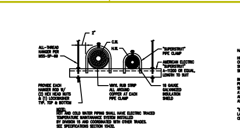
TYPICAL TRAPEZE PIPE HANGER DETAIL N.T.S.
