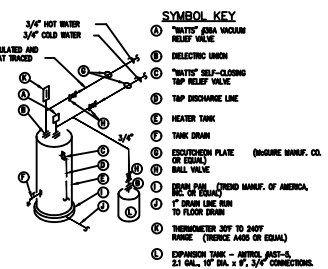
TYPICAL ELECTRIC WATER HEATER PIPING SCHEMATIC N.T.S.
