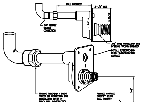
TYPICAL NON-FREEZE WALL HYDRANT DETAIL N.T.S.
