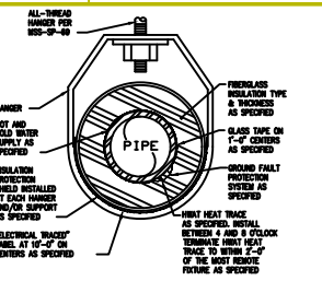
TYPICAL HEAT TRACE DETAIL N.T.S.
